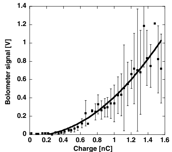
FIG. 2. Bolometer voltage versus charge per bunch for a 30 mrad collection half angle. Each square represents an average of 50 experimental shots, with rms variation as error bar. The solid line is a quadratic fit to the data, indicating coherence of the radiated signal. The bolometer (Infrared Laboratories) had a voltage responsivity S = 2.73 \times 10^8 V/W and thermal conductivity G = 17.01 \mu\text{W/K} . Since the radiation bursts are much shorter than the bolometer time constant, \tau_{\text{bolo}} = 0.33 ms, the detector operates as a calorimeter. The absorbed energy is then given by E_{\text{absorbed}} = G\tau_{\text{bolo}}\Delta V_{\text{bolo}}/(R\eta_{\text{bolo}}) = 4.0\Delta V_{\text{bolo}} (in pJ), where R = SG = 4.64 is the induced voltage per K of temperature rise (in V/K), \Delta V_{\text{bolo}} is the height of the voltage pulse (in V), and \eta_{\text{bolo}} \sim 0.3 is the bolometer efficiency. The radiated energy is E_{\text{radiated}} = E_{\text{absorbed}}/\eta_{\text{coll}} , where \eta_{\text{coll}} is the overall collection efficiency of the system.
