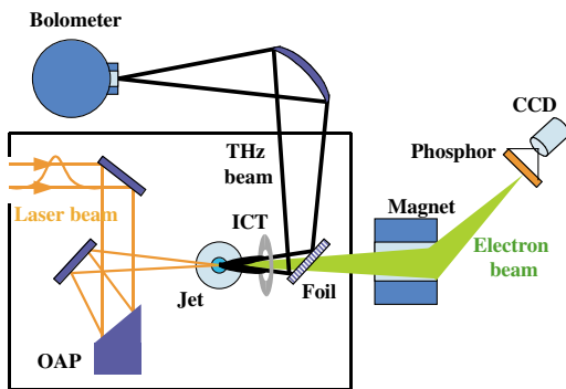
FIG. 1 (color online). Schematic of the experimental setup. High peak power laser pulses entered the vacuum chamber and were focused onto a high pressure pulsed He gas jet using an off-axis parabola (OAP). An integrating current transformer (ICT) measured the amount of accelerated electrons (charge). A metal-coated foil directed the THz radiation outside the vacuum chamber onto a spherical mirror that focused the radiation onto a helium cooled bolometer. The electron energy distribution was measured using an imaging magnetic spectrometer to momentum disperse the e beam onto a phosphor screen that was imaged by a CCD camera.
