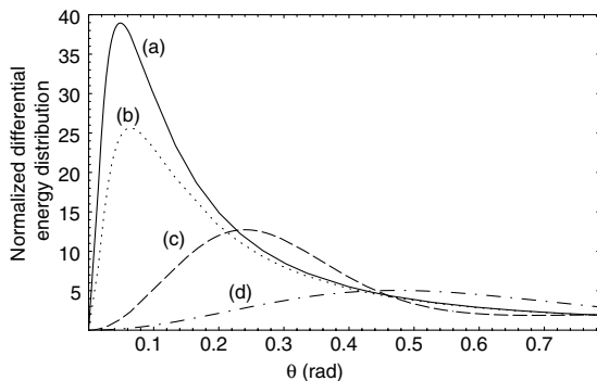
FIG. 3. Normalized energy per unit solid angle and frequency of the coherent radiation (d^2W_e/d\omega d\Omega)\pi^2 c/e^2 N_e^2 versus observation angle \theta for the normalized transverse plasma size \rho/\lambda and e -beam temperature u_T : (a) \rho/\lambda = 100 and u_T = 12 (solid curve), (b) \rho/\lambda = 100 and u_T = 9 (dotted curve), (c) \rho/\lambda = 2 and u_T = 9 (dashed curve), and (d) \rho/\lambda = 1 and u_T = 9 (dot-dashed curve). Curve (d) is near experimental parameters.
